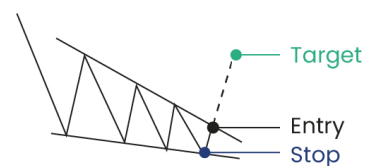
Falling Wedge
