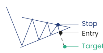
Bearish Penant
