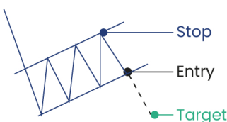
Bearish Flag
