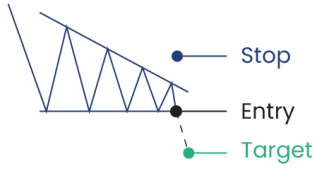
Descending Triangle
