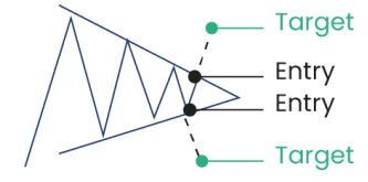
Symmetrical Triangle
